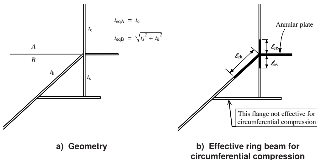
Figure 8.3: Effective section of the cylinder / hopper / ring transition
