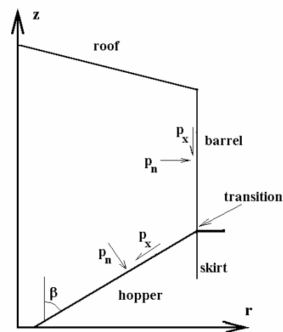
b) silo shell coordinates and loading: section
