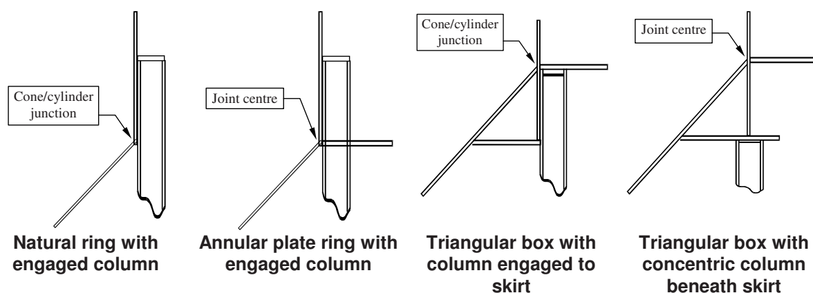
Figure 8.1: Example ring forms
