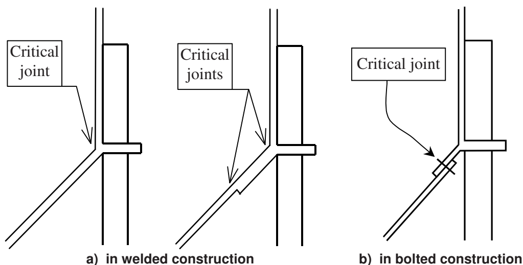
Figure 6.2: Hopper transition joint: potential for rupture
