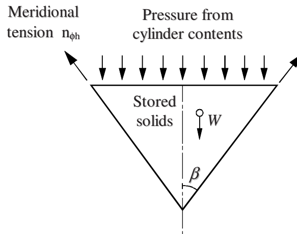
Figure A.1: Hopper global equilibrium
