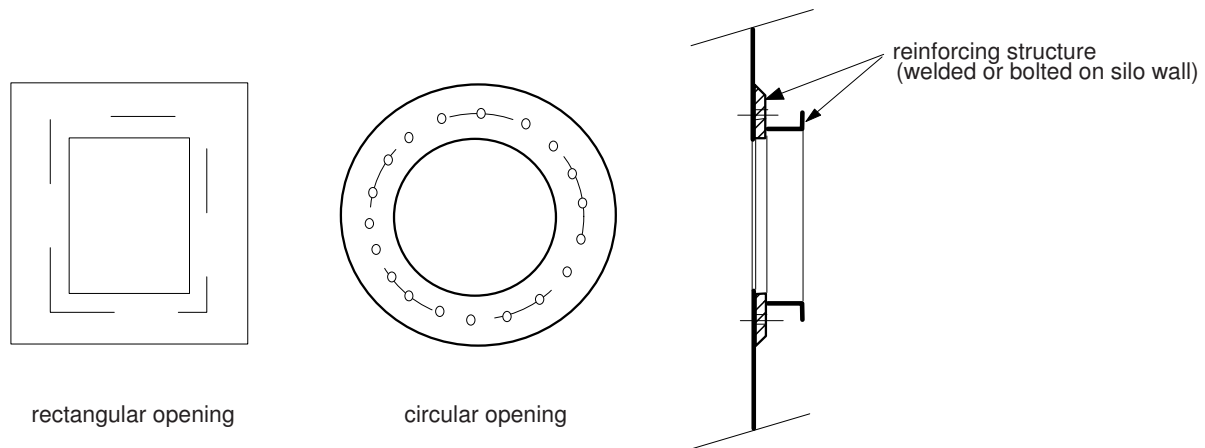
Figure 5.9: Typical stiffening arrangements for openings in silo walls
