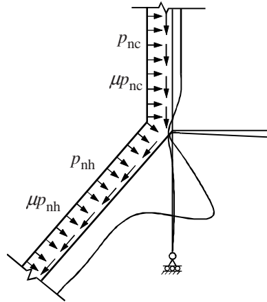
Figure 6.3: Plastic collapse of conical hopper
