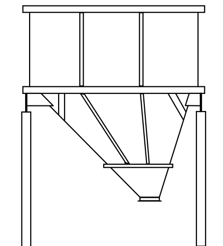
Figure 9.12: Unsymmetrical hopper with inclined ribs
