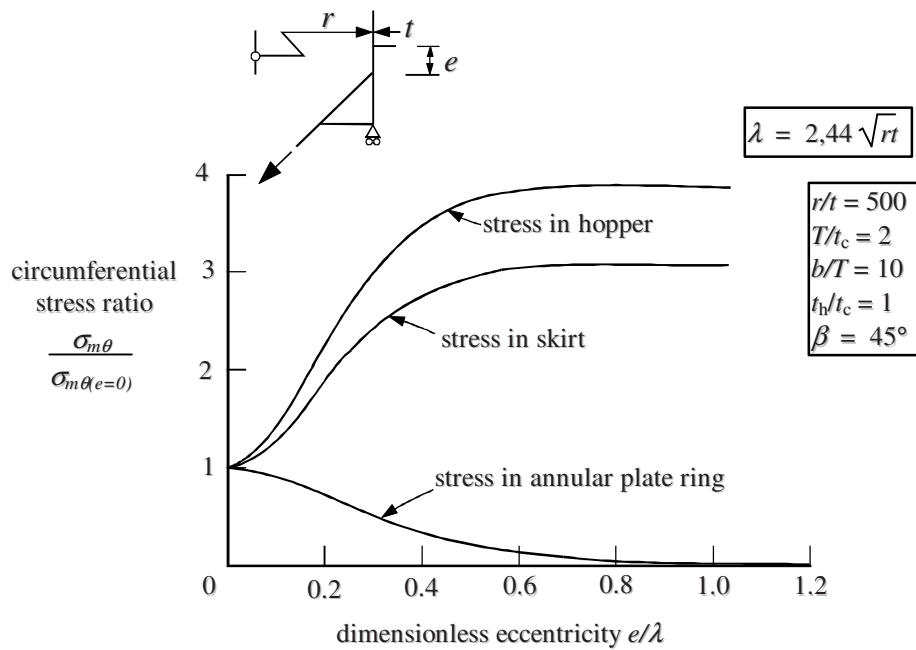
Figure 8.2: Membrane stresses developed in a ring and adjacent shell when the ring is eccentric
