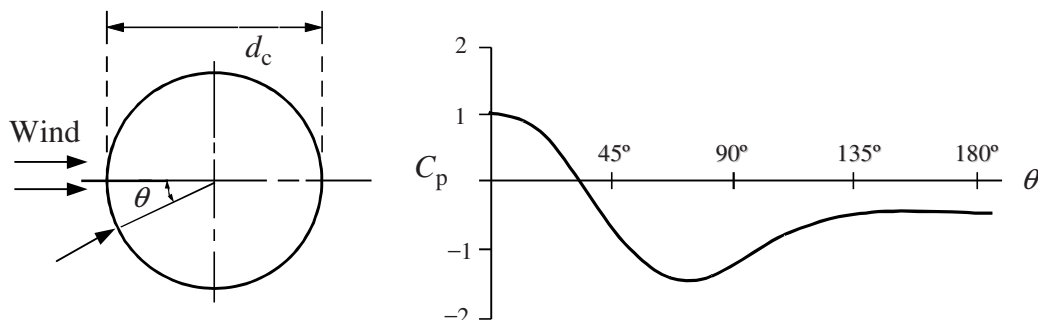
Figure C2: Wind pressure variation around half circumference in isolated silo
