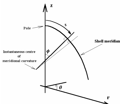
AC1 a) global coordinate system AC1
