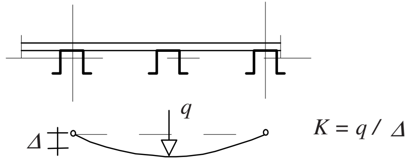
Figure 5.5: Evaluation of restraint stiffness against stiffener column buckling
