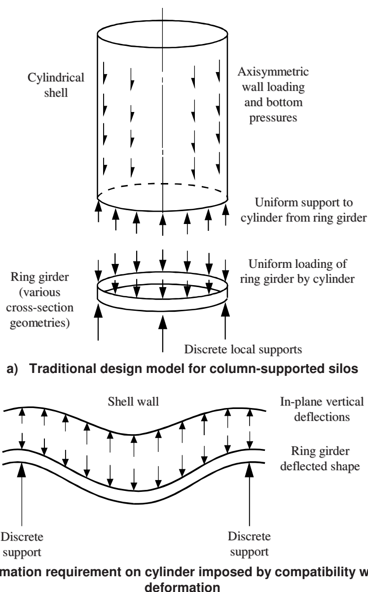
Figure 4.1: Axial deformation compatibility between ring girder and shell
